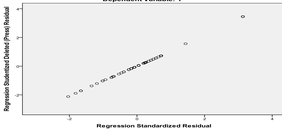
Scatterplot Dependent Variable: Y
