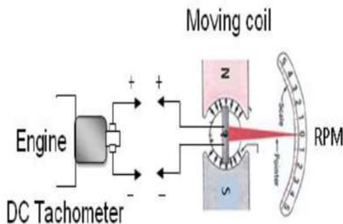
Gambar 2.13. Tachometer DC
