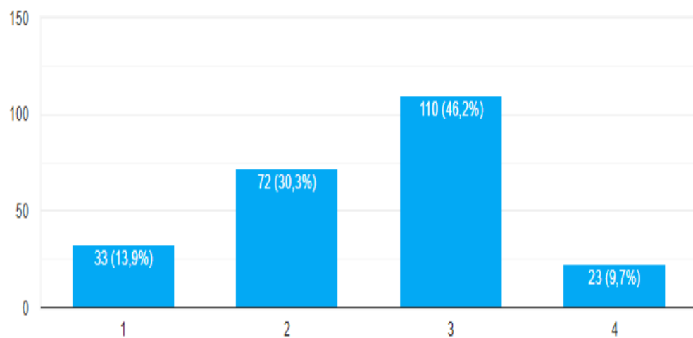
Gambar lampiran 8. Histogram variabel X8
