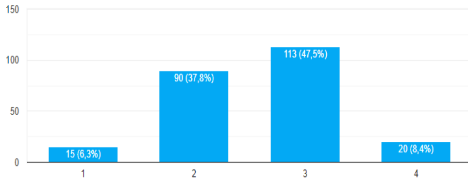
Gambar lampiran 5. Histogram variabel X5
