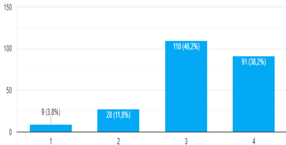
Gambar lampiran 16. Histogram variabel Y8
