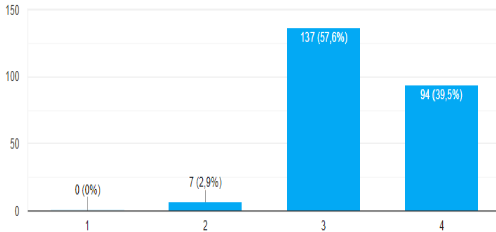
Gambar lampiran 1. Histogram variabel X1
