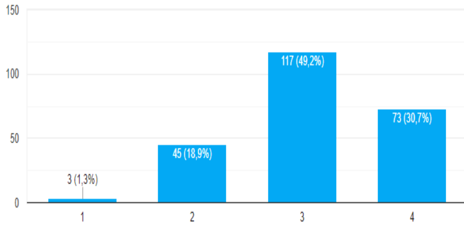
Gambar lampiran 11. Histogram variabel Y3
