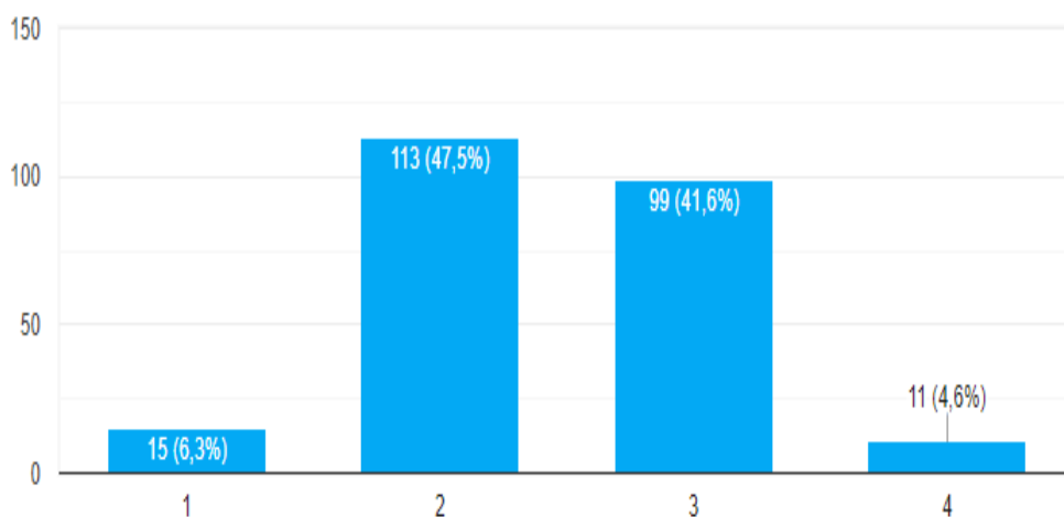
Gambar lampiran 2. Histogram variabel X2
