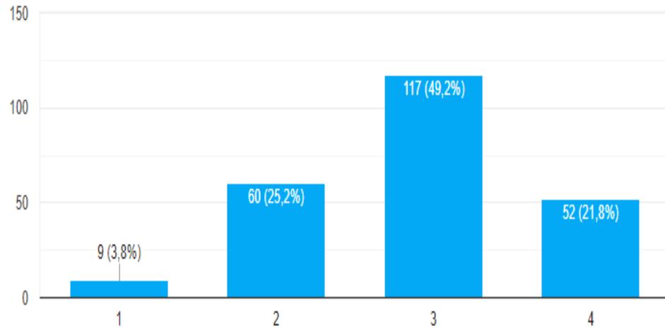
Gambar lampiran 15. Histogram variabel Y7
