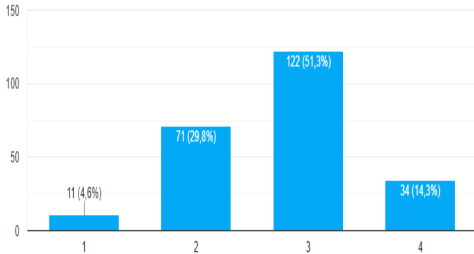
Gambar lampiran 7. Histogram variabel X7
