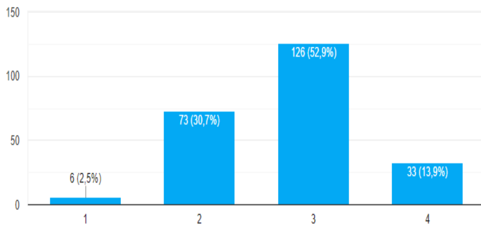
Gambar lampiran 6. Histogram variabel X6
