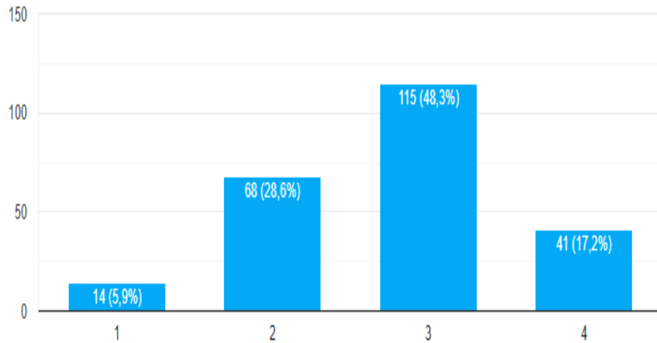
Gambar lampiran 9. Histogram variabel Y1
