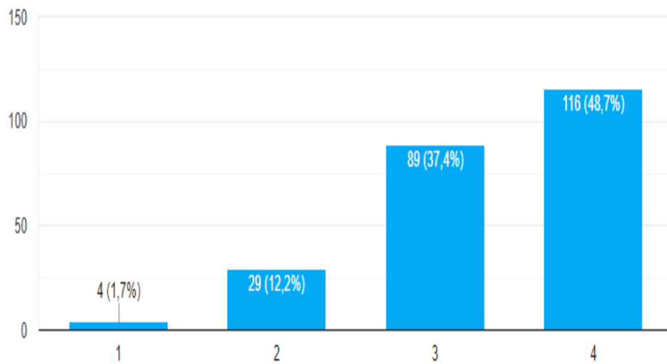
Gambar lampiran 12. Histogram variabel Y4
