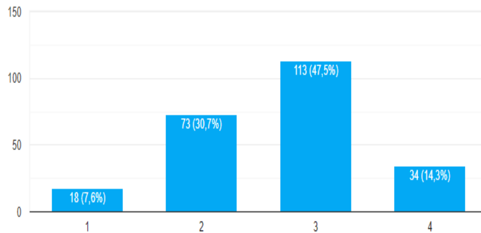
Gambar lampiran 10. Histogram variabel Y2
