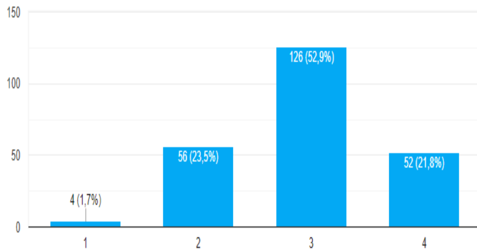
Gambar lampiran 14. Histogram variabel Y6
