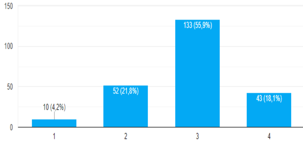
Gambar lampiran 13. Histogram variabel Y5
