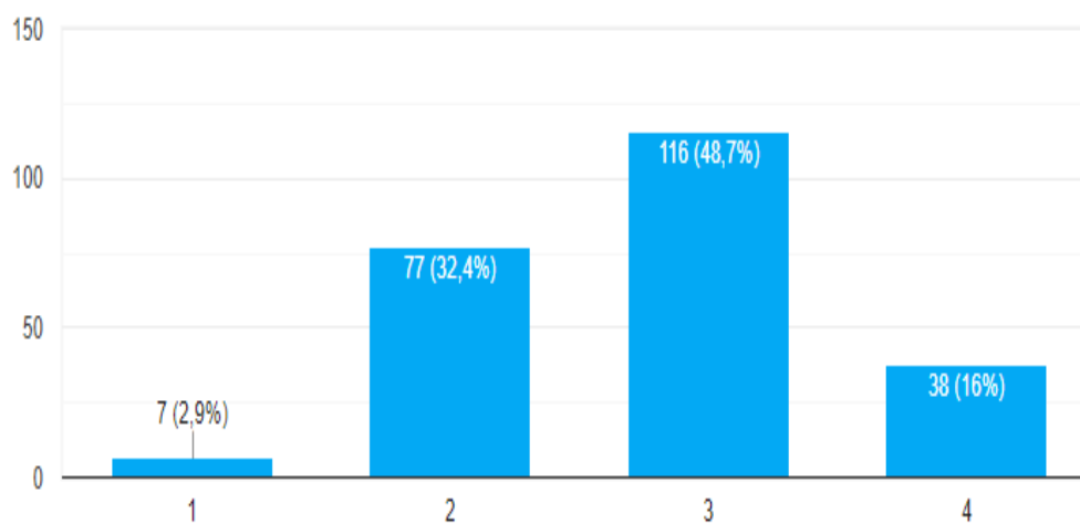
Gambar lampiran 4. Histogram variabel X4
