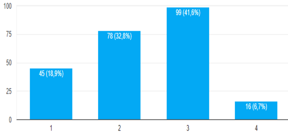
Gambar lampiran 3. Histogram variabel X3
